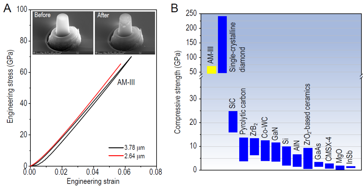
Figure 4. Compressive strength of AM-III compared with other known materials. (A) Engineering stress-strain curves recorded during uniaxial compressing AM-III micropillars. The insets are the SEM images of the pillar with diameter of 3.78 \mu\text{m} before and after compression. There was almost no size change, but some wrinkles produced on upper part of the pillar are like the shear bands formed in metallic glasses [3]. (B) Comparison of compressive strength for various materials with micron size [34–36]. The results demonstrate that AM-III is strongest amorphous materials known to date.
