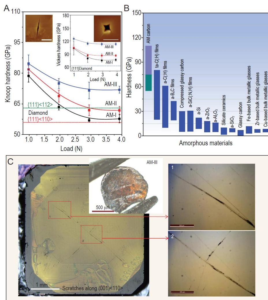
Figure 3. Hardness of AM carbon materials, compared with other known amorphous materials, and scratches on diamond (001) face indented by AM-III. (A) H_K as a function of applied loads. Left inset: AFM image of Knoop indentation of AM-III after unloading from 3.92 N. Right inset: H_V of AM carbon materials as a function of applied load and AFM image of Vickers indentation of AM-III sample after unloading from 2.94 N. The scale bars in indentation images are 10 \mu\text{m} . Error bars of hardness indicate s.d. ( n = 5 ). The dashed lines indicate H_V and H_K of (111) plane of natural diamond crystal. (B) Hardness of different amorphous materials [1,4,8,11,33]. Green and violet columns indicate H_K and H_V of AM carbon materials, respectively. Considering the hardness of film materials are characterized by nanoindentation hardness ( H_N ), the H_N of AM carbon materials was also measured, and AM-III has high H_N of 103 GPa, exceeding that (80.2 GPa) of ta-C films [8]. (C) Scratches on the (001) face of diamond by using AM-III sample displayed in the inset as an indenter (left image), indicating the ultrahard nature of AM-III. The zoomed-in right images are corresponding to the areas marked by red rectangles in the left image, displaying the scratches in more detail.
