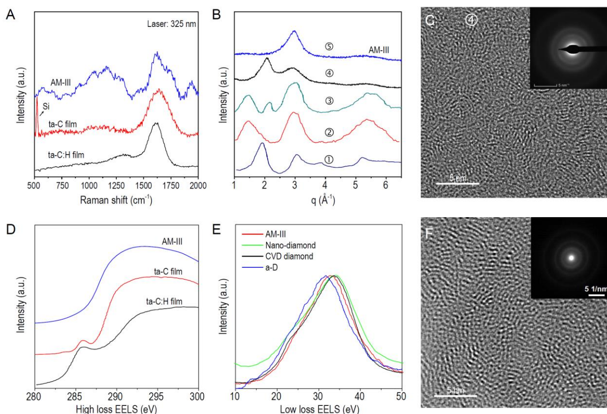
Figure 6. Comparison of AM-III currently discovered with other AM carbon materials. (A) Raman spectra show AM-III has an obvious T-band around 900\sim 1300\text{ cm}^{-1} compared to ta-C(:H) films [8,27]. (B) XRD patterns of various AM carbon materials recovered from compressing \text{C}_{60} at p,T conditions: ① 8 GPa, 1200^\circ\text{C} [17]; ② 12.5 GPa, 500^\circ\text{C} [17]; ③ 13.5 GPa, 1000^\circ\text{C} [17]; ④ 15 GPa, 800^\circ\text{C} (our data); ⑤ 25 GPa, 1200^\circ\text{C} (AM-III, our data). (C and F) HRTEM images and SAED patterns of the material synthesized at p,T condition ④ and compressed GC [11], respectively. (D) High loss EELS of AM-III and ta-C(:H) films [46,47]. (E) Low loss EELS demonstrating the plasmon peak position in AM-III, a-D [12], CVD diamond [48], and nano-diamond [49].
